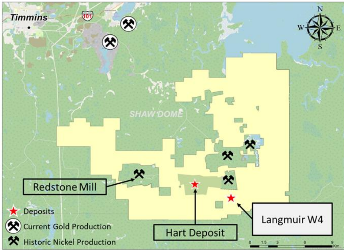
Figure 1: Location of Langmuir W4 Zone in the Shaw Dome
