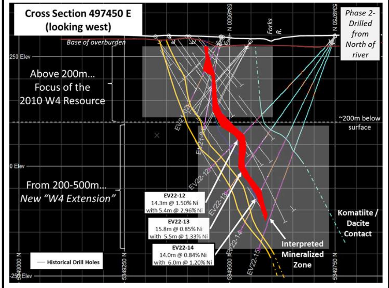
Figure 2: Target Area for the New "W4 Extension"
